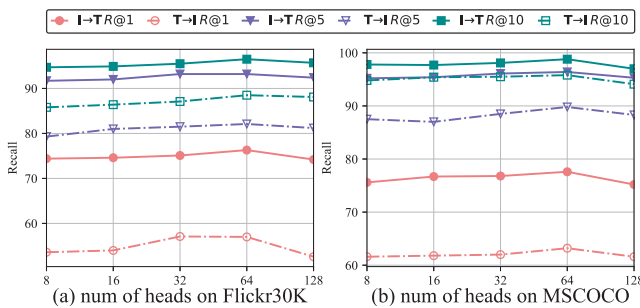
Figure 3: Evaluation of heads number k .
