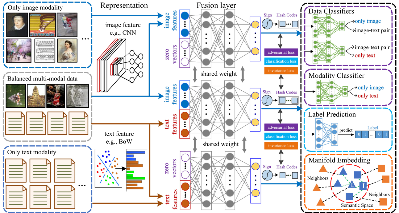
Fig. 2. The schematic pipeline of the proposed ATFH-N framework, which can handle both balanced and imbalanced multi-modal data.
