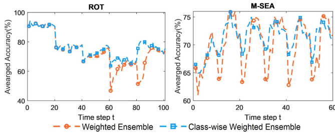
Fig. 6. Averaged prediction accuracy over 20 independent runs of Class-wise weighted ensemble and weighted ensemble on M-SEA and ROT data sets.
