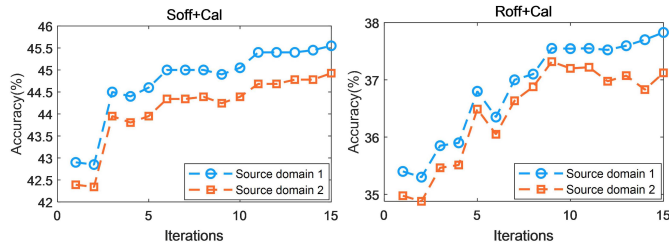
Fig. 8. Prediction accuracy(%) along with the iteration of AW-CORAL.
