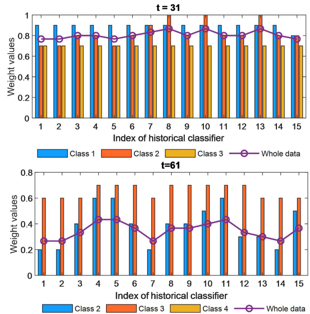
Fig. 7. Weights of historical classifiers on each class and the whole data chunk when t = 31 and t = 61 .
