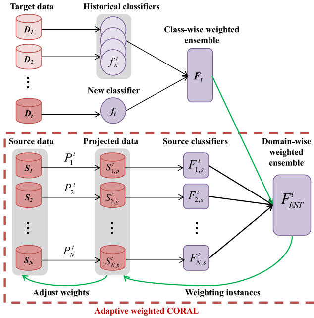
Fig. 2. Framework of the proposed hybrid ensemble approach to a concept drift-tolerate transfer learning problem at the t -th time step.
