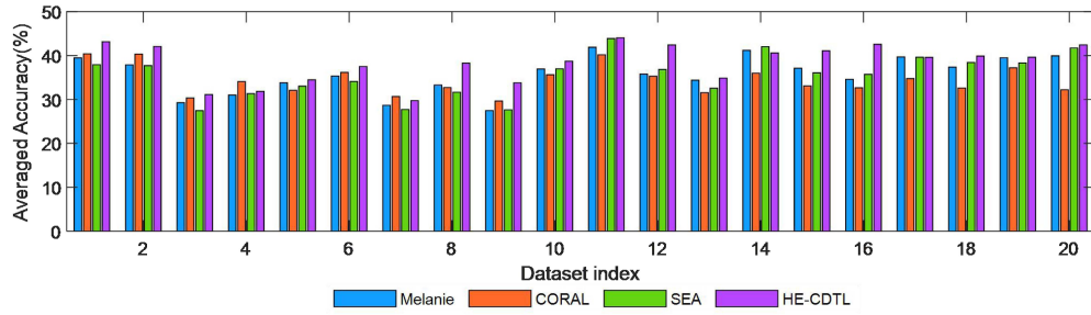
Fig. 5. Averaged prediction accuracy(%) over 20 independent runs of Melanie, CORAL, SEA, and HE-CDTL on RPIE, SPIE data sets.
