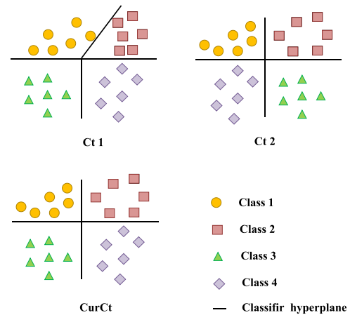
Fig. 1. Illustration of different shifts among classes. Ct 1 and Ct 2 are the two historical concepts, and CurCt is a concept at the current time step. The drift between Ct 1 and CurCt exists in Class 1 and Class 2. The drift across the Ct 2 and CurCt only causes the labels of Class 3 and Class 4 swapping.
