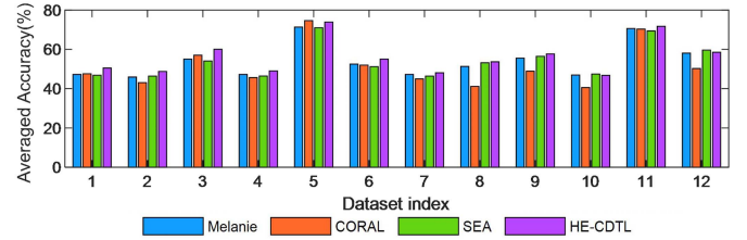
Fig. 4. Averaged prediction accuracy(%) over 20 independent runs of Melanie, CORAL, SEA, and HE-CDTL on ROff+Cal, SOff+Cal data sets.
