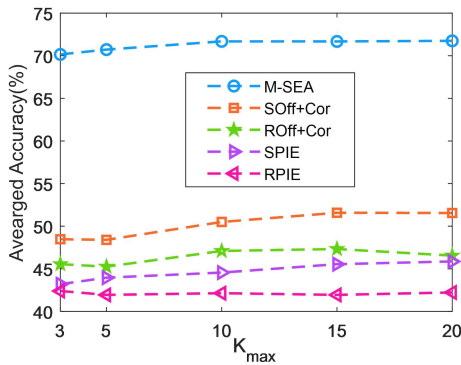
Fig. 9. Averaged prediction accuracy over 20 independent runs of HE-CDTL with different K_{max} on five cross-domain tasks.
