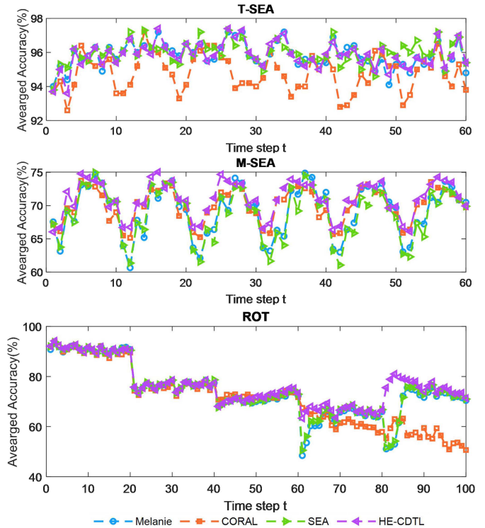
Fig. 3. Averaged prediction accuracy over 20 independent runs of Melanie, CORAL, SEA, and HE-CDTL on three synthetic data sets.
