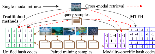
Fig. 8. The illustration of different hash representation for single-modal retrieval and cross-modal retrieval tasks.
