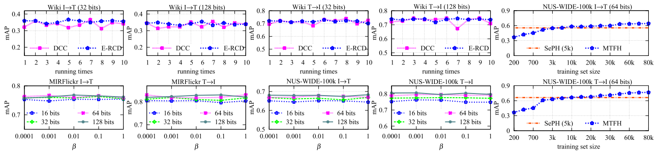
Fig. 9. Effects of different optimization schemes, parameter values and training set sizes.
