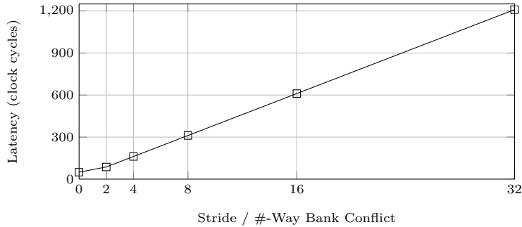
Fig. 5. Latency of Fermi Bank Conflict
