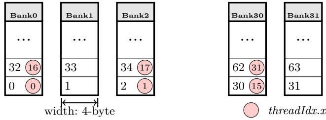
Fig. 4. Fermi Shared Memory Banks
