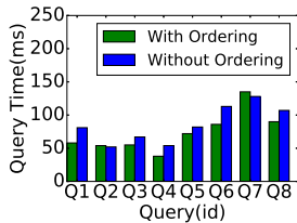
Fig. 17: Specialization order optimization
