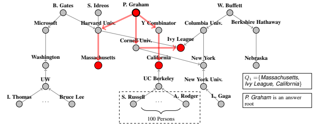
Fig. 1: An example data graph G , a keyword search Q_1 and its answer (red)
