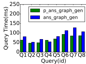
Fig. 18: Path-based answer generation optimization
